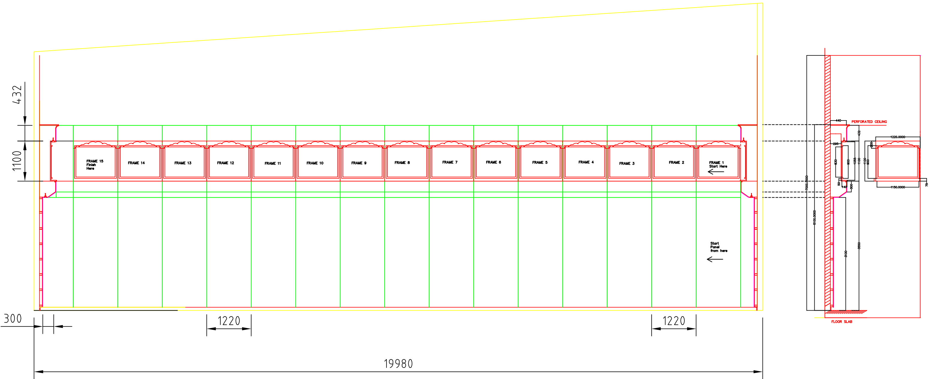
SOUTH SIDE ELEVATION Revision 3 (17-06-12)
