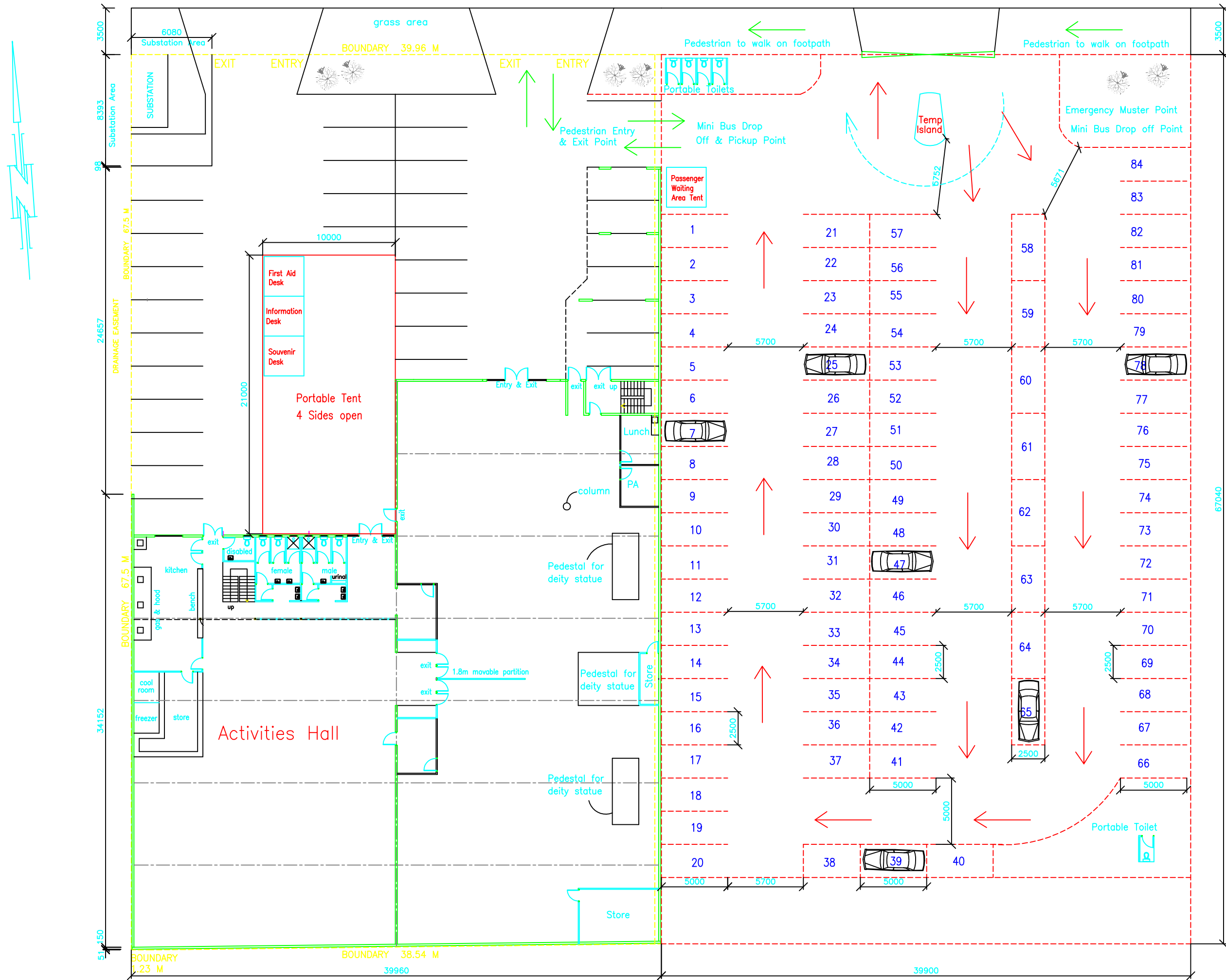
SITE/GROUND FLOOR PLAN
